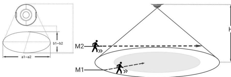
Fig.3.3.2(1)Installation diagram of CSBP-04/00.1.0x and CSBP-04/00.2.0
