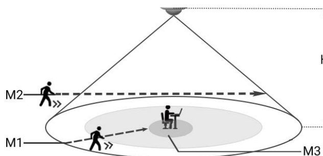
Installation diagram of CSBPM-04/00.1.0x and CSBPM-04/00.2.0x
