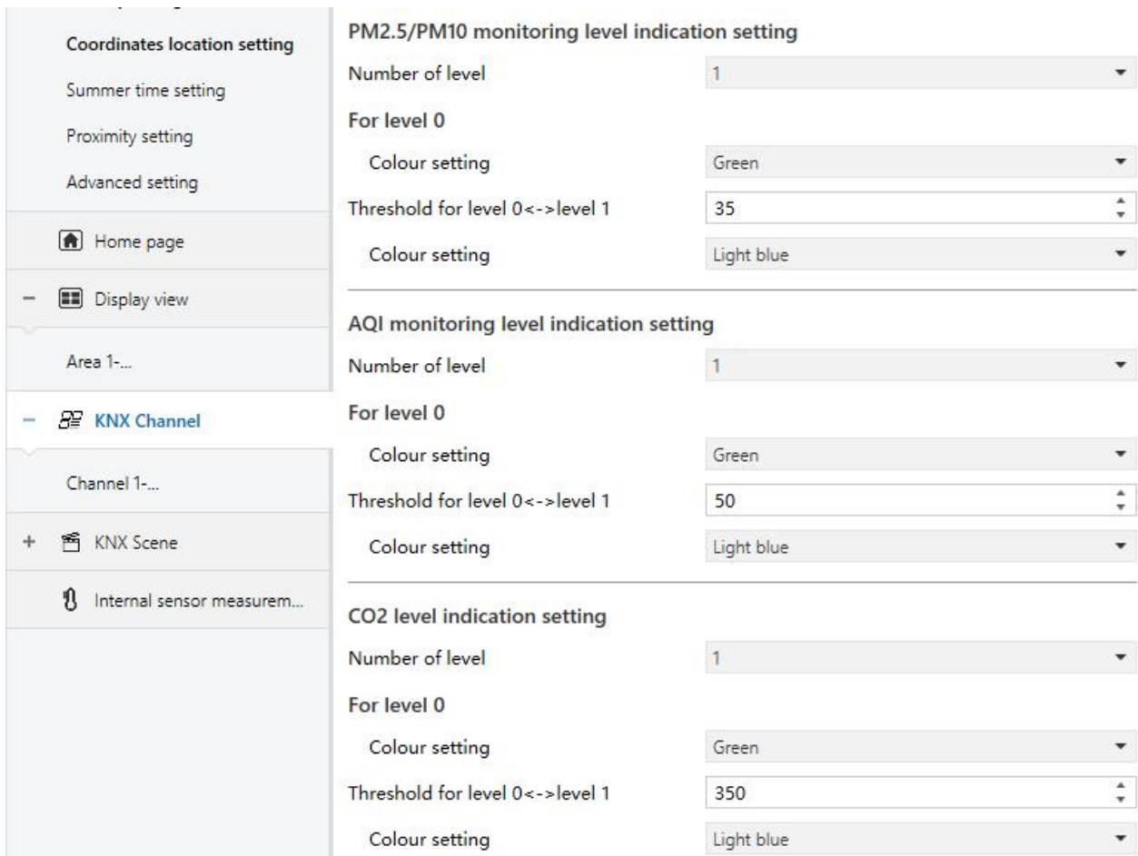
Fig.5.11 “KNX Channel”parameter window
