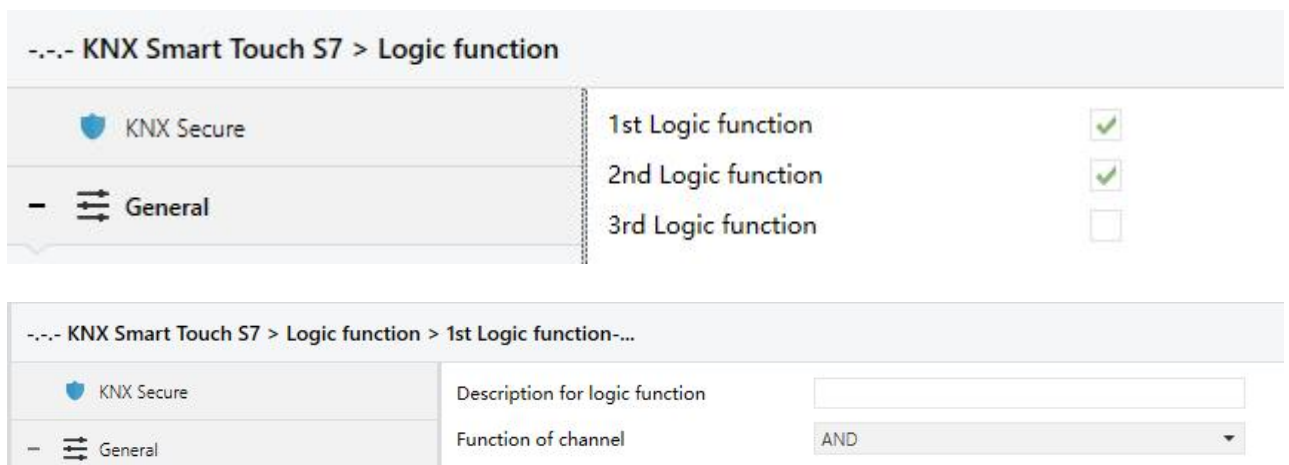
Fig.5.7 "Logic function"parameter window
