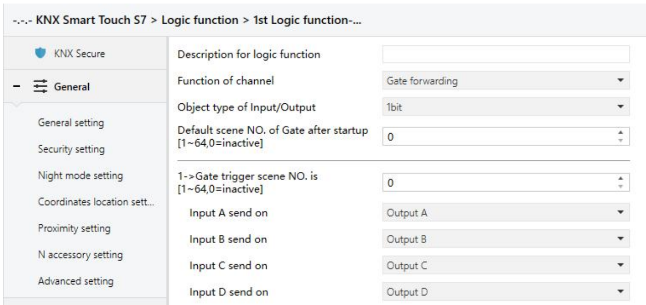
Fig.5.7.2 "Logic function_Gate forwarding" parameter window
