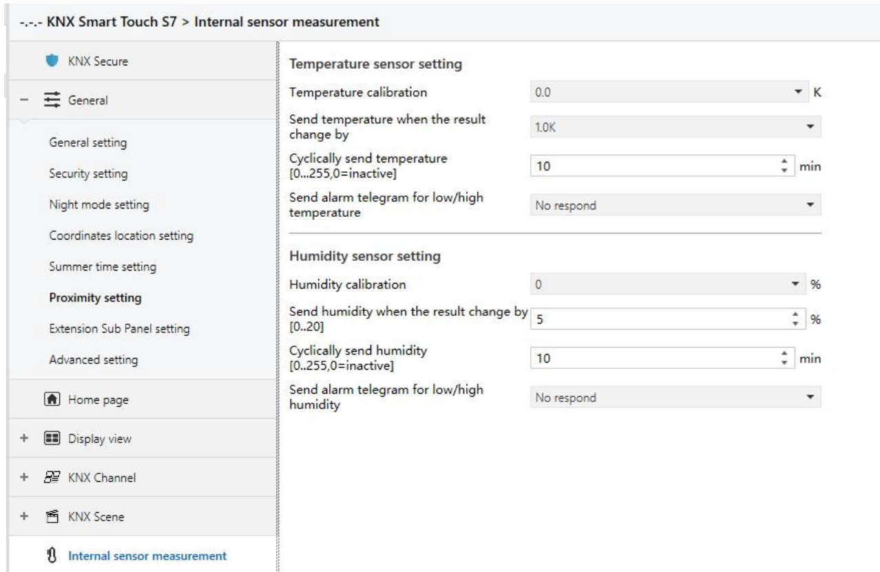
Fig.5.13 "Internal sensor measurement"parameter window
